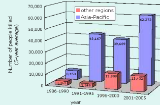
Number of people killed by water-related disaster
